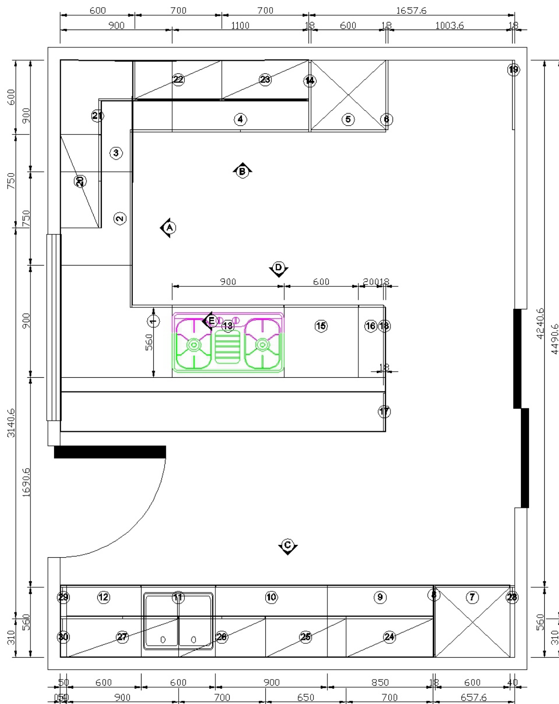
Plan drawing
