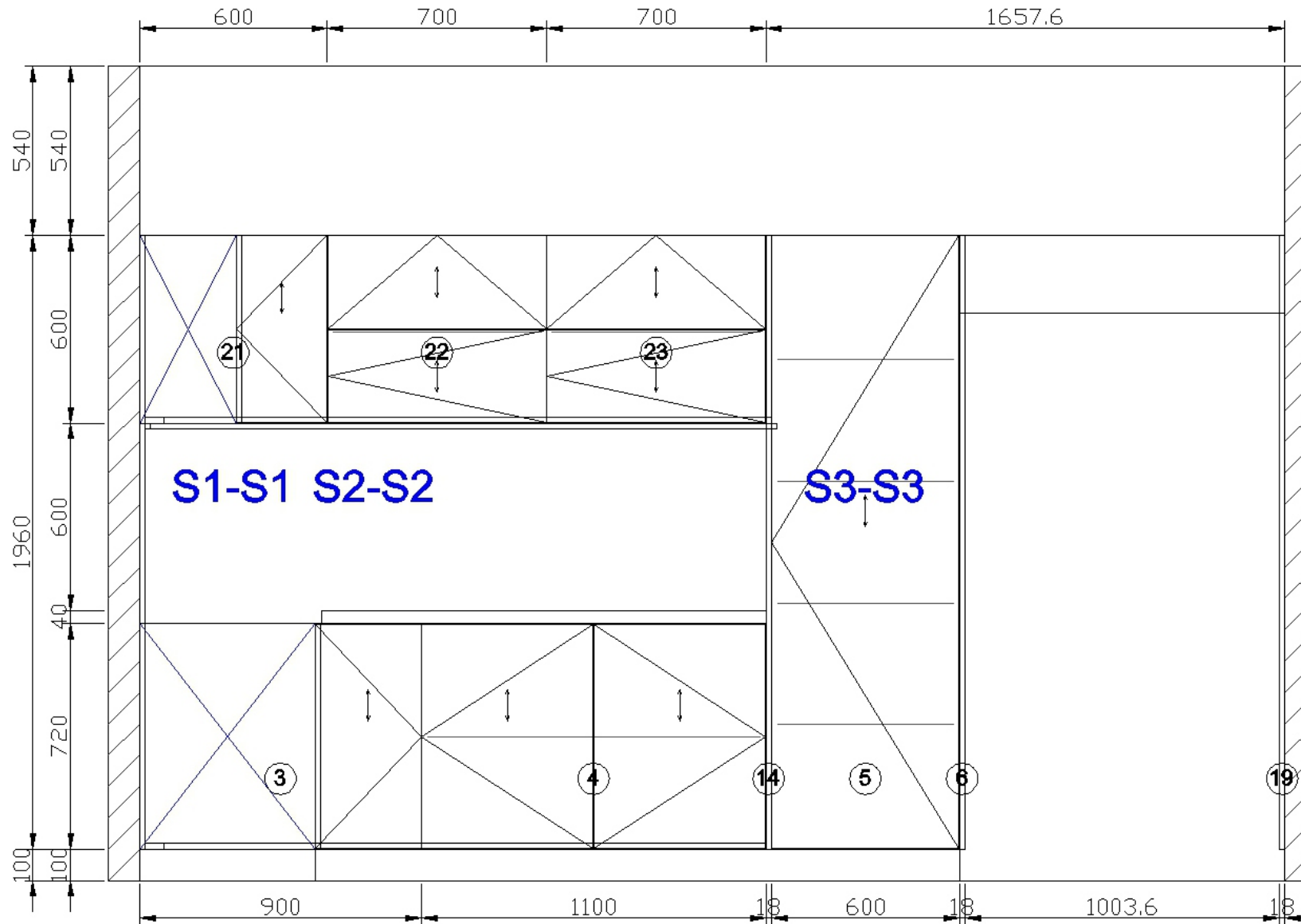
B View elevation drawing
