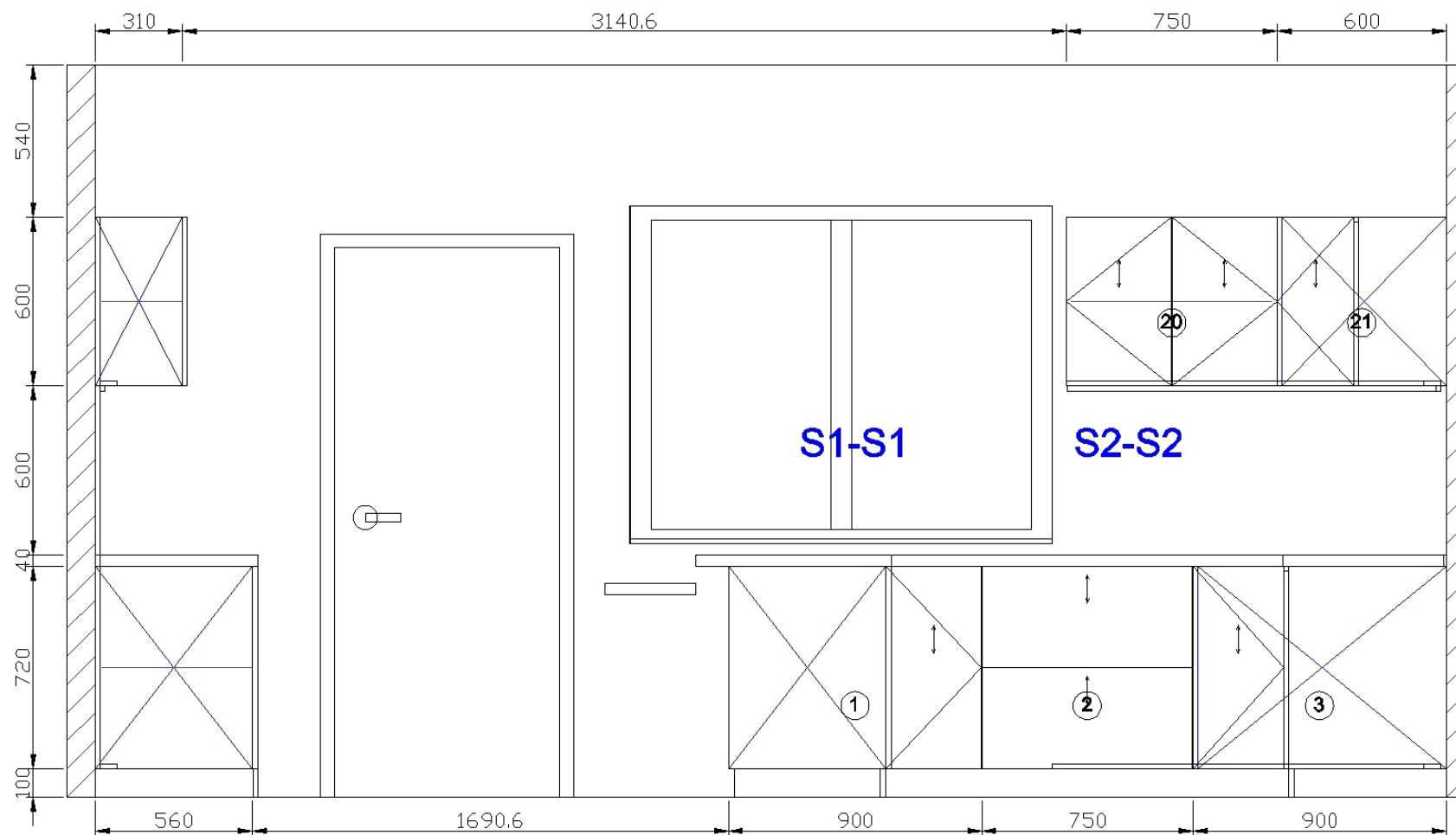
A View elevation drawing
