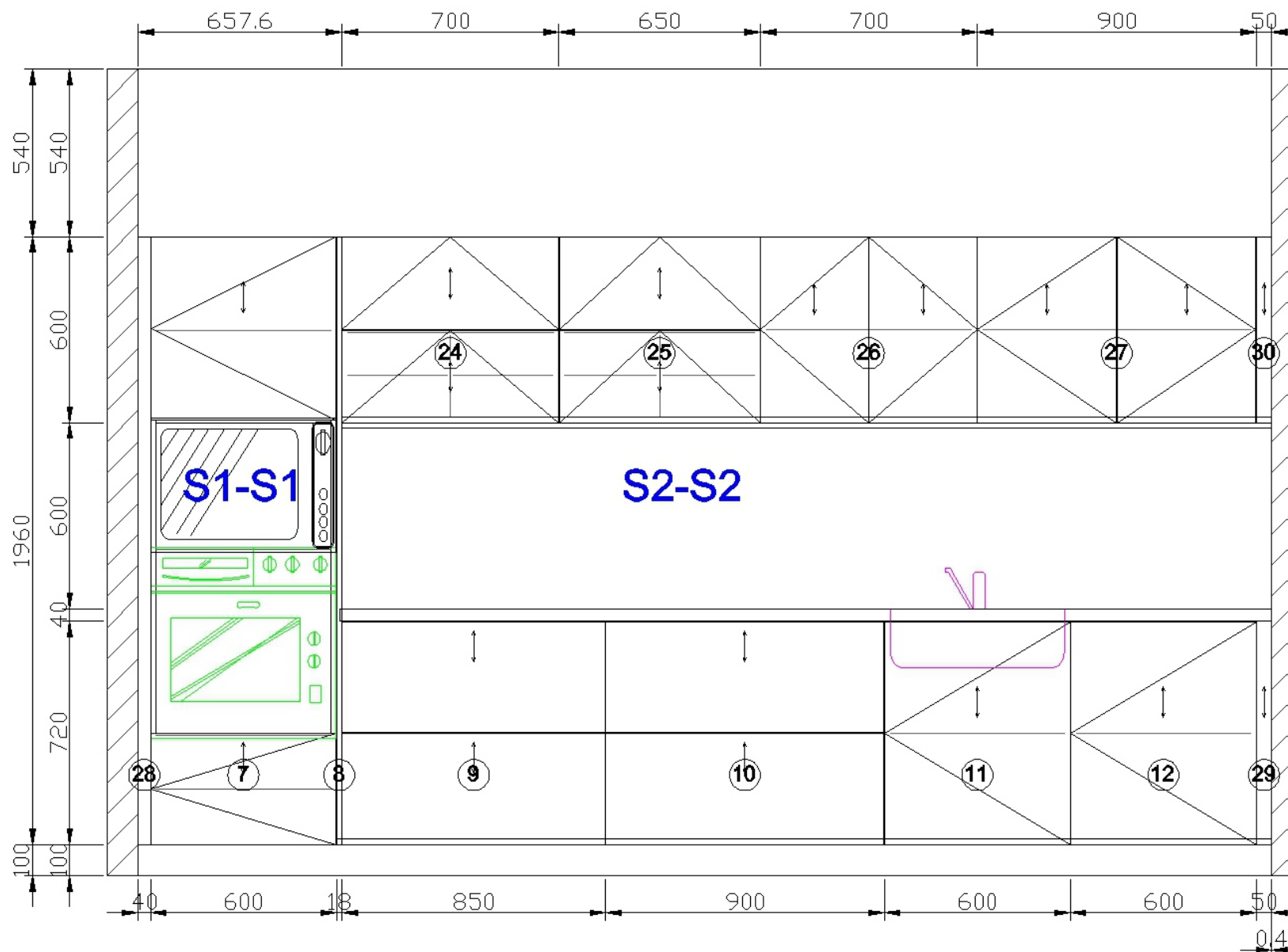
C View elevation drawing
